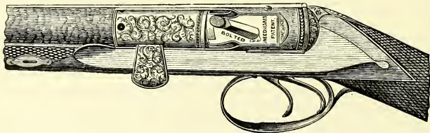
Needham's Central-fire Needle Gun.
